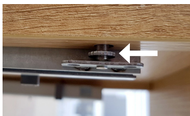
Adjusting nut on underside of drawers.
